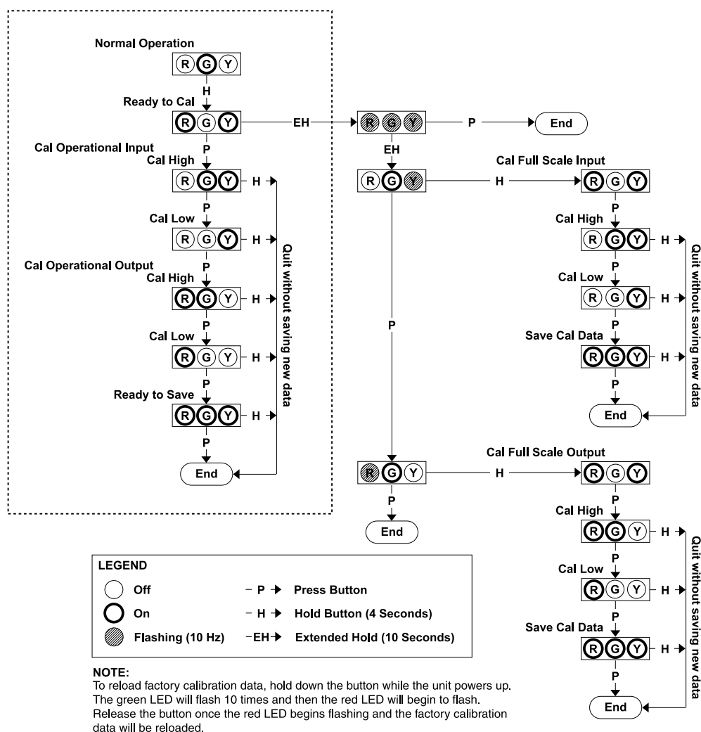
Figure 3: Switch Settings
